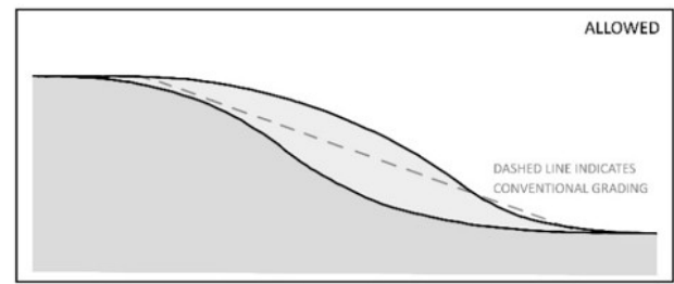
LANDFORM GRADING - SLOPES VARY (TWO OPTIONS SHOWN)
