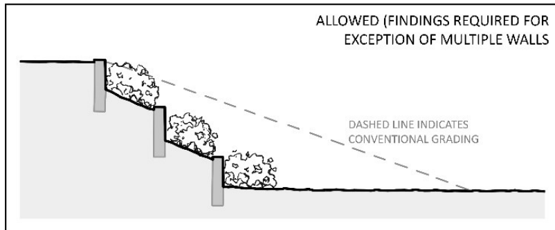
MULTIPLE RETAINING OR GARDEN WALLS WITH TERRACED PLANTING (MAXIMUM 8')
