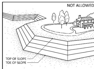
CONVENTIONAL GRADING
